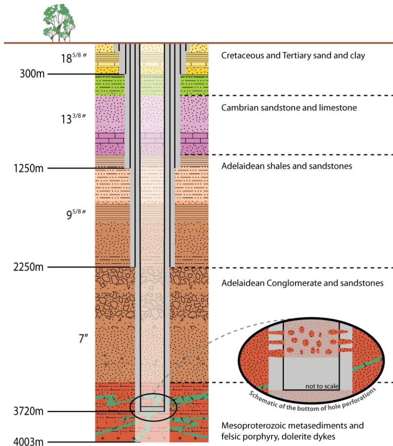
Figure - Paralana well 2 – fracture stimulation zone and target interval
